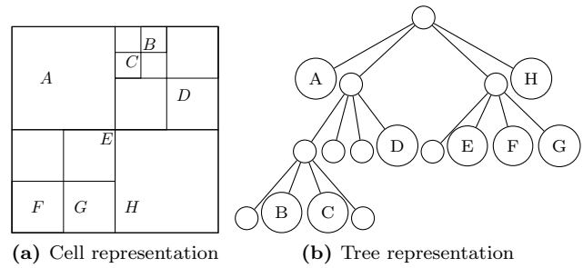
Figure 2: Visual representations of the same Barnes-Hut tree. ( http://arborjs.org/docs/barnes-hut )
