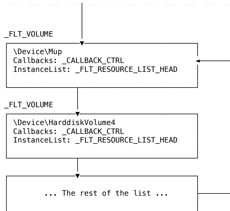
(Fig 3) Association between _FLT_FRAME and _FLT_VOLUME
