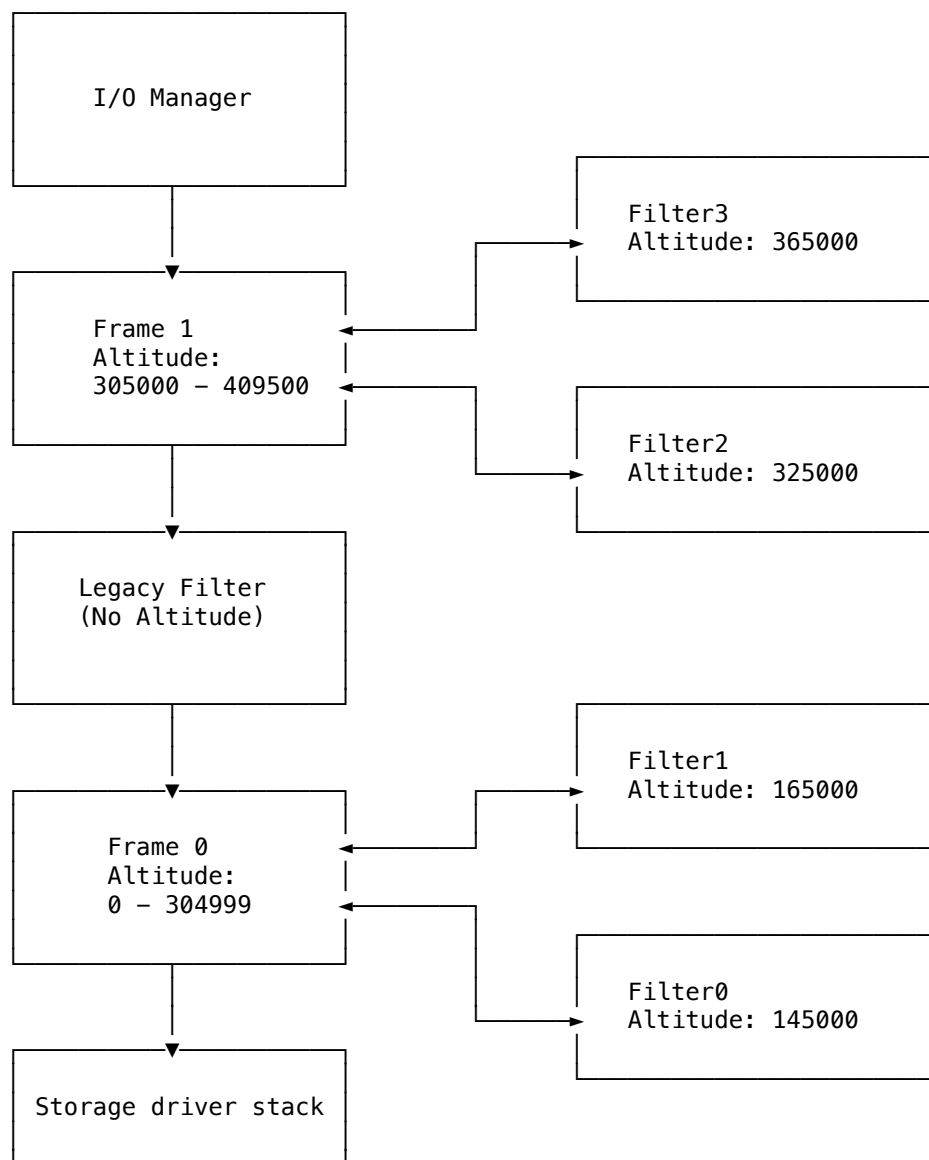
(Fig 2) Simplified version of figure 2: https://learn.microsoft.com/en-us/windows-hardware/drivers/ifs/filter-manager-concepts
